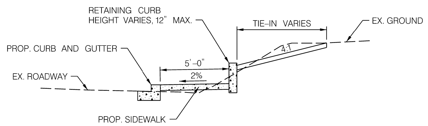
TYPICAL SIDEWALK SECTION WITH BACK CURB ALONG CHESTNUT AVE.
