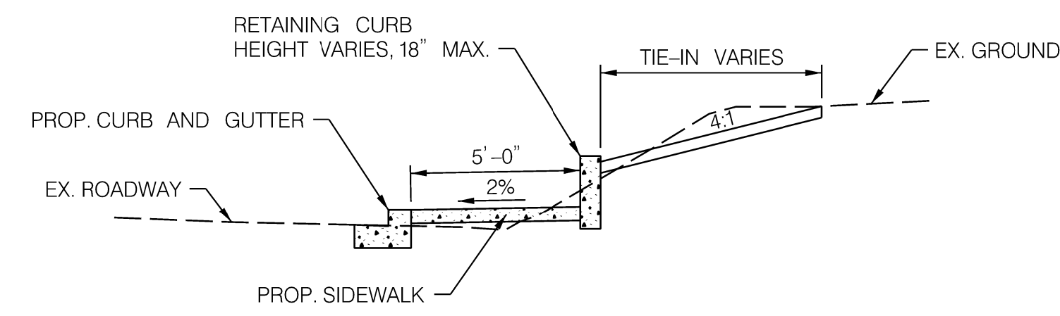
TYPICAL SIDEWALK SECTION ALONG CHESTNUT AVE.
